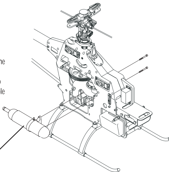
Fuel Filter (not included)
