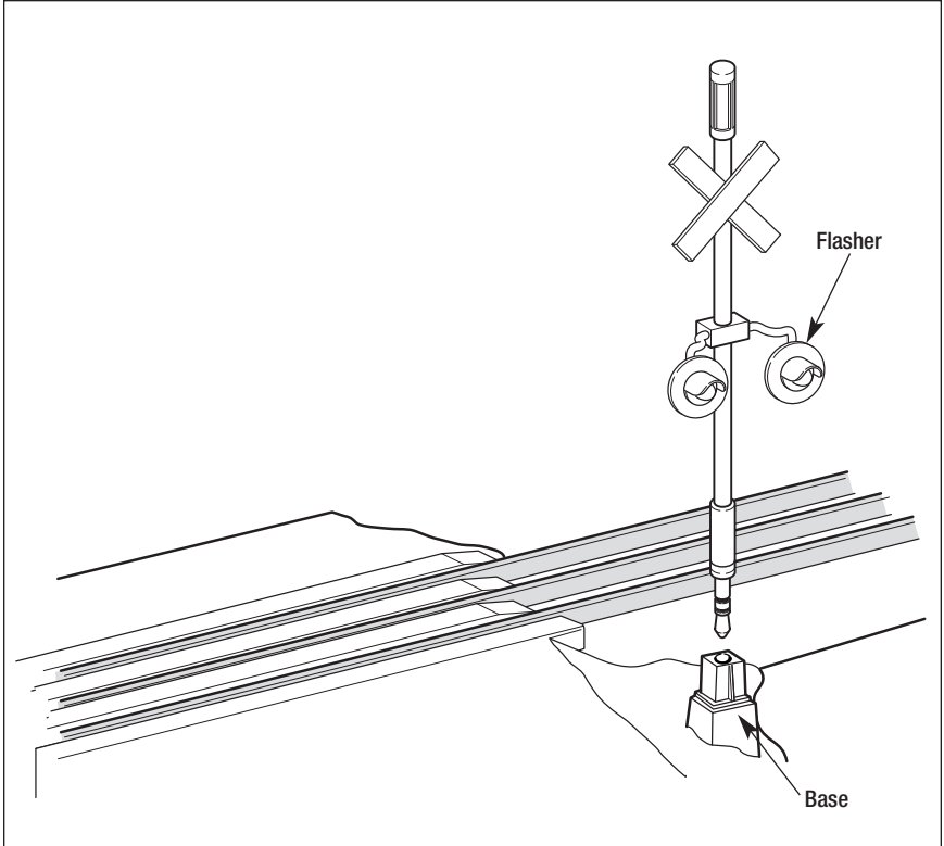
Figure 3. Flasher installation
